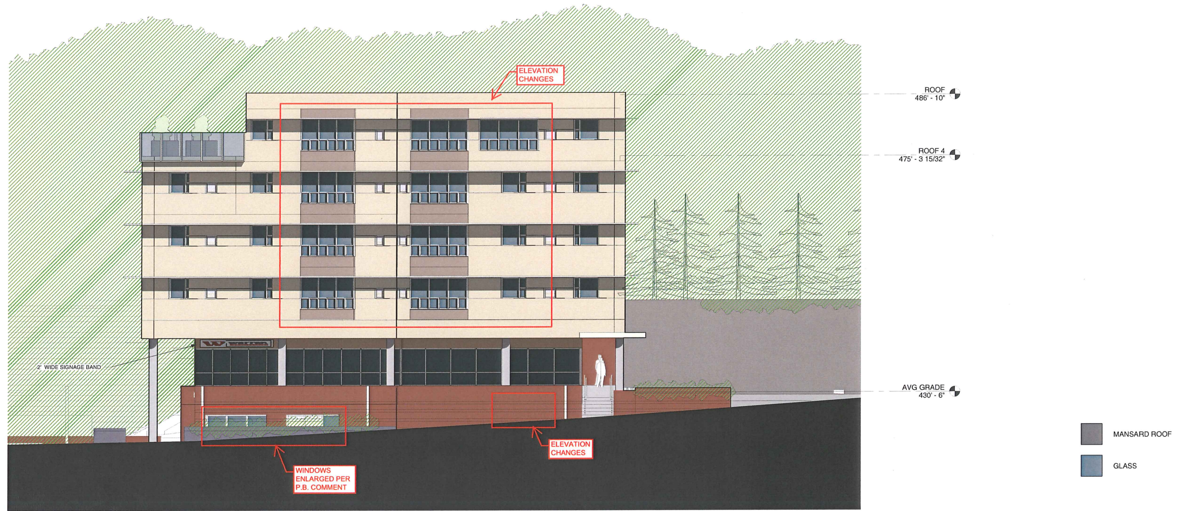
1 SOUTH ELEVATION 1/8" = 1'-0"
