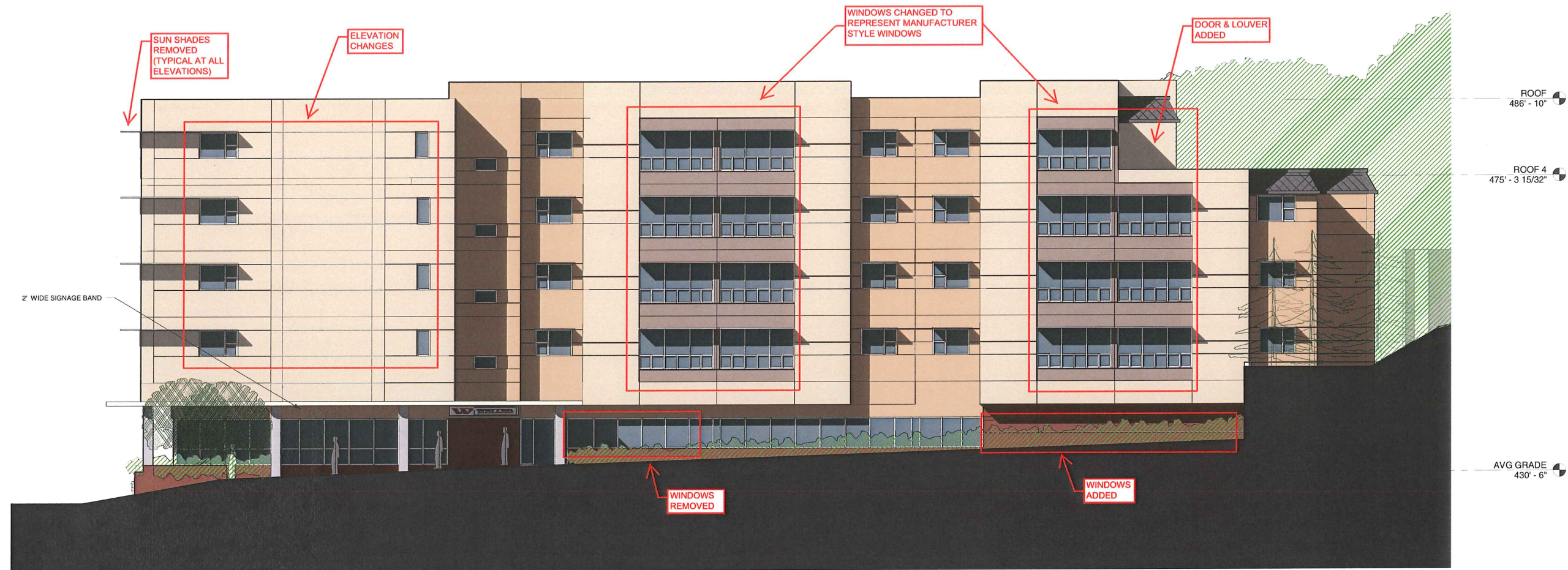
1 EAST ELEVATION 1/8" = 1'-0"
