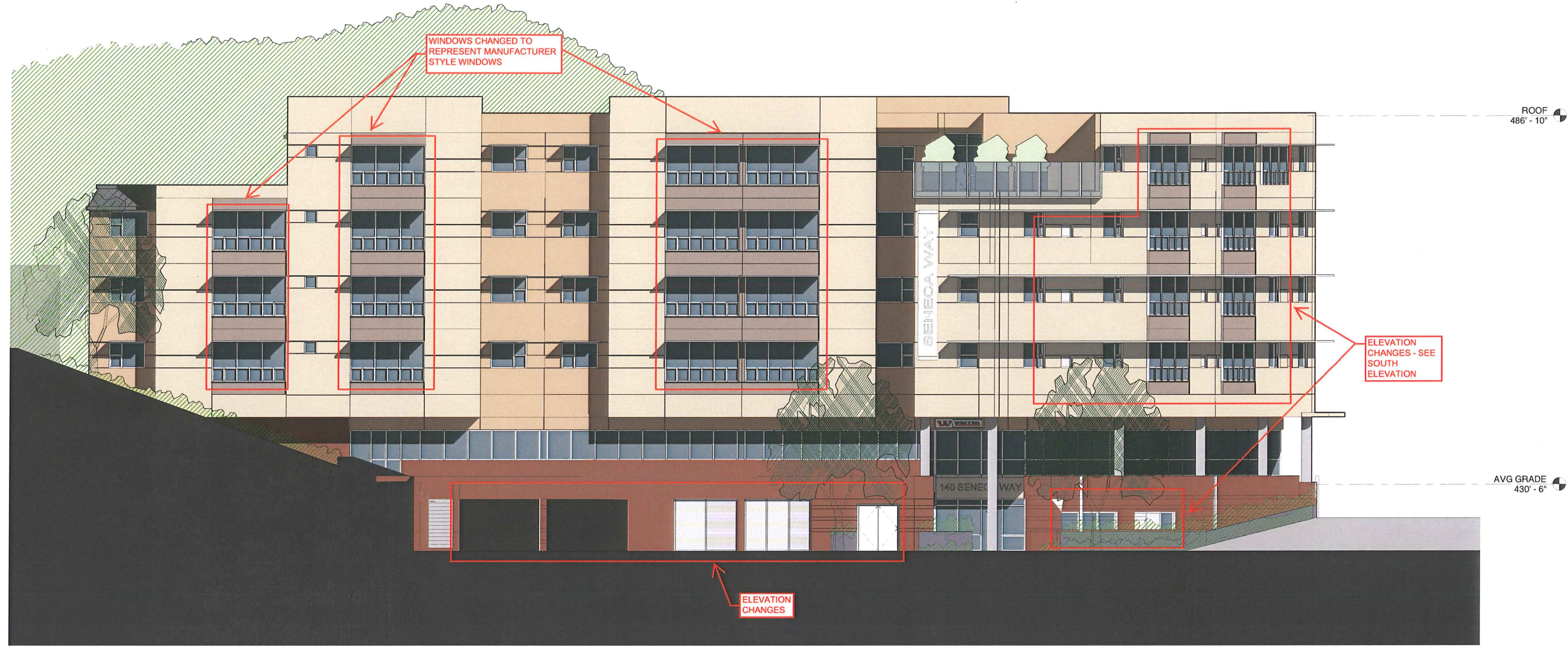
2 WEST ELEVATION 1/8" = 1'-0"
