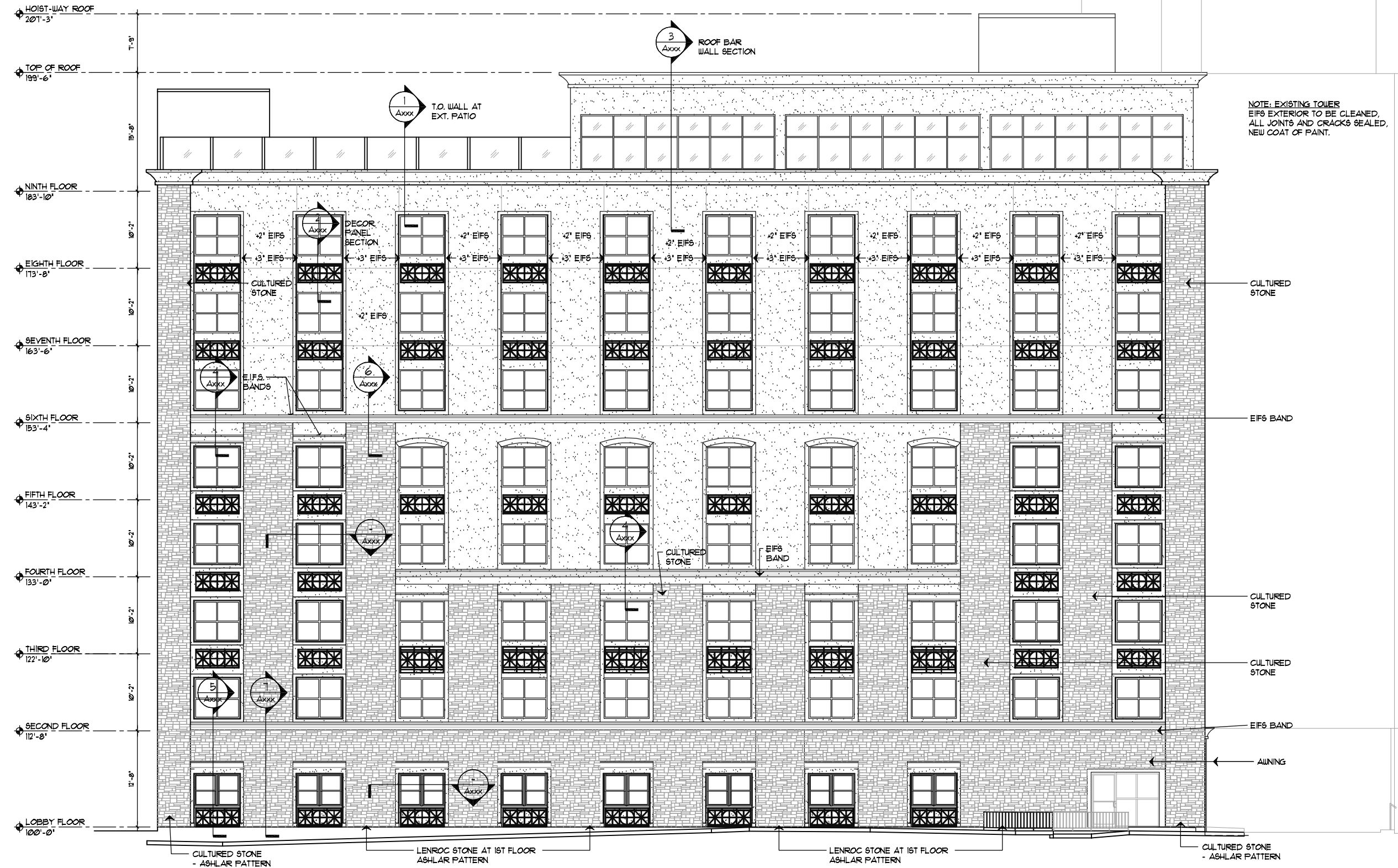
1 SOUTH EXTERIOR ELEVATION SCALE: 1/8" = 1'-0"
